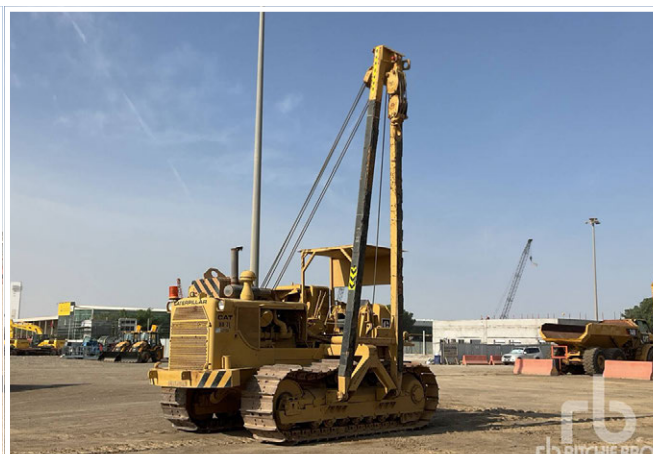
1 / 4, CAT 583K
