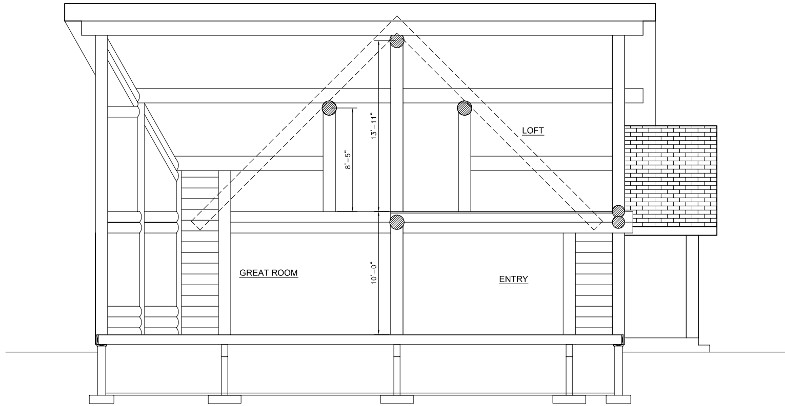
CROSS SECTION
