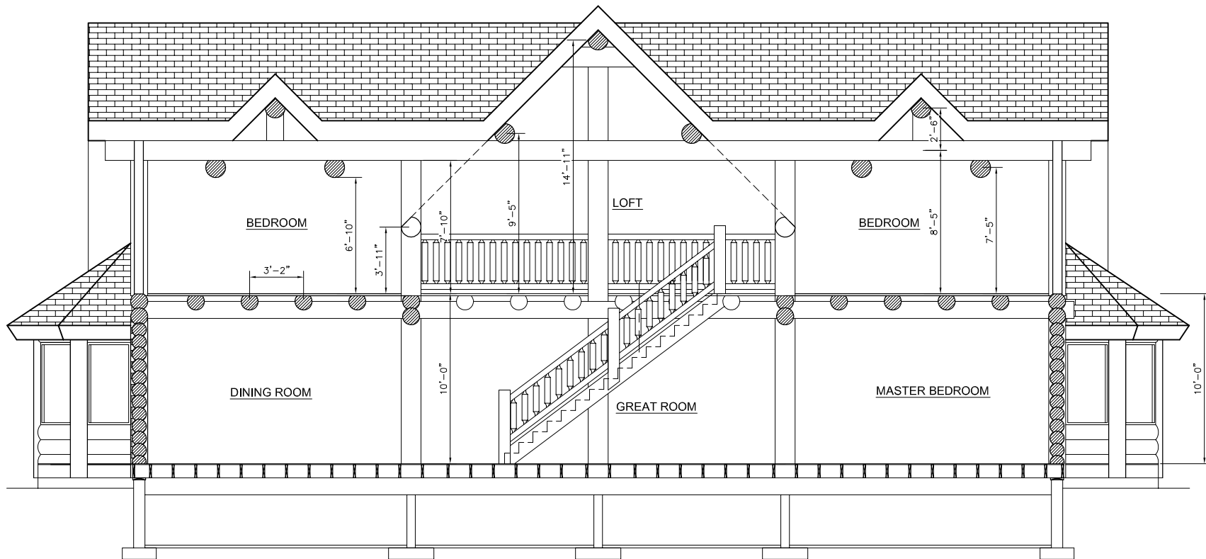
TRANSVERSE SECTION
