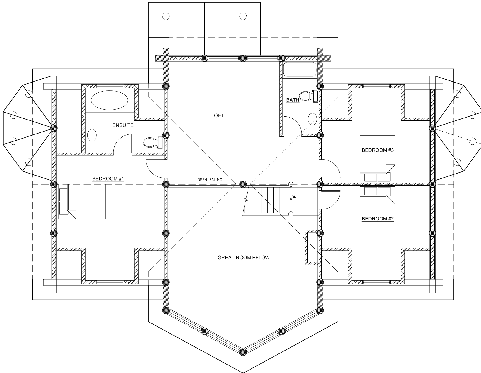
2 PROPOSED SECOND FLOOR PLAN (1080 SF) A1 SCALE 1/4" = 1'-0"
